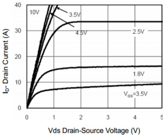
Figure 3 Output Characteristics
