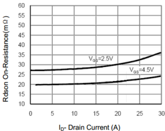
Figure 5 Drain-Source On-Resistance
